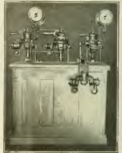
FIG. 3.—"BROWN'S PULPIT."
